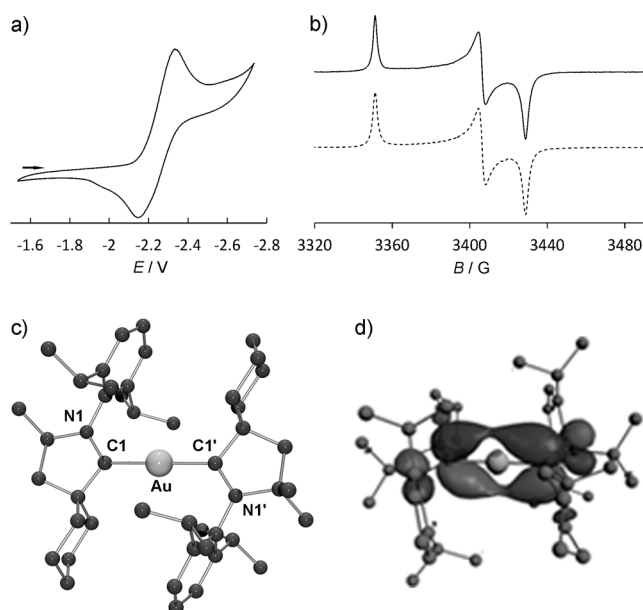
Figure 1. a) Cyclic voltammogram of 1 ( n\text{Bu}_4\text{NPF}_6 as electrolyte, potential versus \text{Fc}^+/\text{Fc} , scan rate 100\text{ mVs}^{-1} ). b) Experimental (—) and simulated (----) EPR spectrum of 2 in a frozen benzene solution at 235 K. B = magnetic field. c) Solid-state structure of 2 (hydrogen atoms are omitted for clarity). Selected bond lengths (Å) and angles ( ^\circ ), with calculated values at (U)M05-2X/def2-SVP in square brackets: Au1–C1 1.991(2) [2.006], C1–N1 1.344(3) [1.348]; C1–Au1–C1' 180 [180]; N1–C1–C1'–N1' 180 [180]; d) Graphical representation of the SOMO of 2 .
