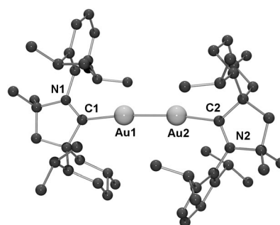
Figure 2. Solid-state structure of 4 with only one rotamer shown (hydrogen atoms are omitted for clarity). Selected bond lengths (Å) and angles ( ^\circ ), with calculated values at M05-2X/def2-SVP in square brackets: Au1–Au2 2.5520(6) [2.579], Au1–C1 2.082(10) [2.123], Au2–C2 2.088(9) [2.133], C1–N1 1.261(12) [1.307], C2–N2 1.337(10) [1.308]; C1–Au1–Au2 173.8(2) [171.3], C2–Au2–Au1 171.3(3) [169.3]; N1–C1–C2–N2 177.65(66) [146.0].
