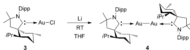
Scheme 2. Synthesis of [(\text{CAAC})_2\text{Au}_2] complex 4 .
