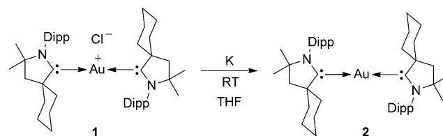
Scheme 1. Synthesis of [(\text{CAAC})_2\text{Au}] complex 2 . Dipp = 2,6-diisopropylphenyl.
